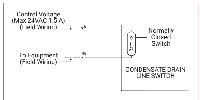
FIG. 5: WIRING DIAGRAM
